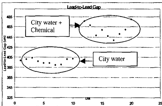
Fig. 15 Lead-to-lead gap characteristic after adding chemical into the city water
