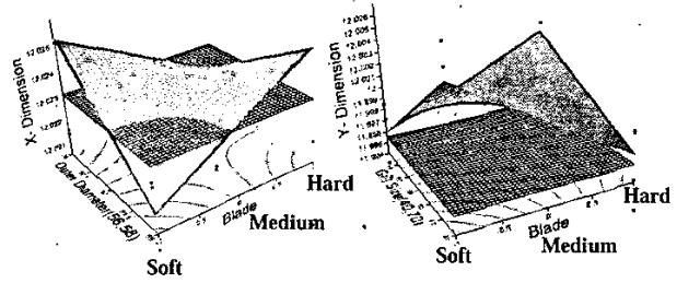
Fig. 5 X-Y dimension to Blade Type, OD & Grit Size Characteristic
