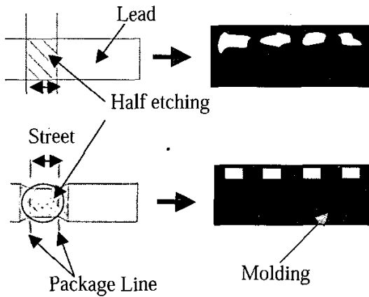
Fig. 3 Substrate Design
