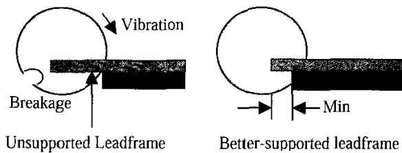
Fig. 4 Less Vibration Mold design
