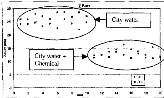
Fig. 13 Z-Burr characteristic after adding chemical into the city water
