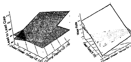
Fig. 10 Lead Gap and Wear Rate to Chilled Water Temperature, Cutting Depth and Feed Rate Characteristic.
