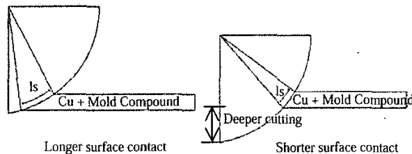
Fig. 17 Contact length difference to substrate by different cutting depth
