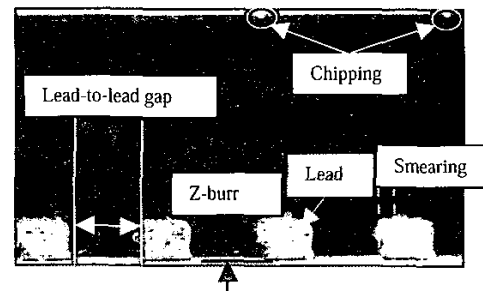
Fig. 2 Cutting Quality
