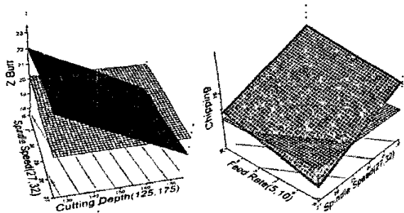
Fig. 9 Z-Burr and Chipping to Spindle Speed, Cutting Depth and Feed Rate Characteristic
